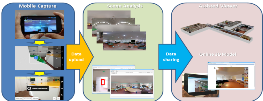
Fig. 2. Mobile Capture module: an interactive mobile application to capture and generate a spherical image for each room, map the multi-room structure by tracking the user movement and recover metric information. Scene Analysis module: a scene analysis tool to reconstruct the 3D model and to create a navigable scenegraph. Assisted Viewer module: a client/server viewer based on WebGL to navigate inside the 3D model through an assisted navigation interface.
