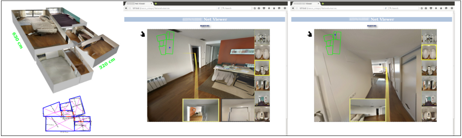
Fig. 5. Left: top view of the 3D scene reconstructed by our system (T3 Tab 1). Center and right: screenshots of interactive browsing of the scene through the Viewer module. The client/server architecture has been defined to achieve a platform independent navigation system running on standard web browsers.
