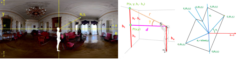
Fig. 3. Left: The equirectangular image represent all possible views for an observer ideally located in the center of the spheremap, identified by the angles \theta and \gamma . Center: h_e is the physical height of the center of the equirectangular image (the ideal eye of the observer) and it is the only value externally entered and not automatically estimated. h_t is the height of the targeted point in respect to the floor plane. Right: The transformation G_h returns real Cartesian coordinates if the height h is known.
