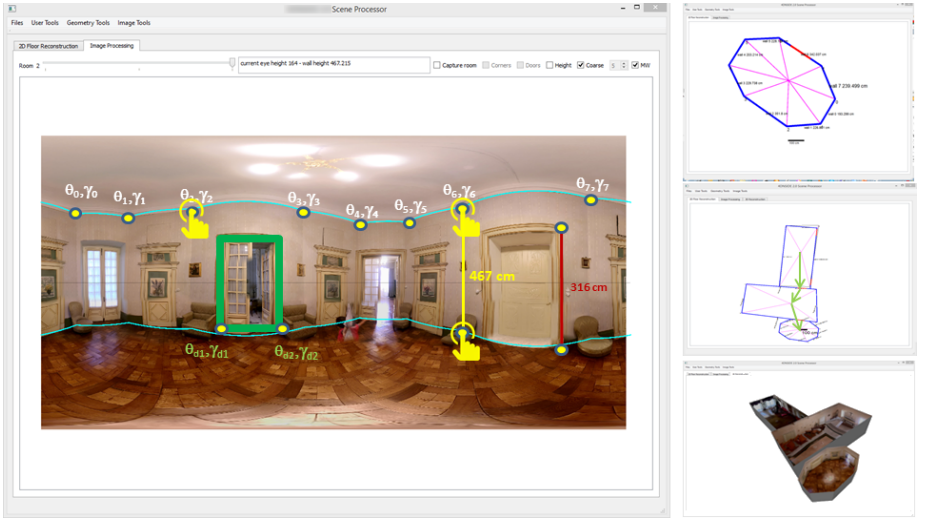
Fig. 4. Server side interface. Left: this tool enables several preliminary scene analysis tasks, like metric measurements on the image (i.e. wall height in yellow, door height in red) and room’s corners identification starting from the automatic boundaries detection (i.e. cyan contours). Top right: reconstruction in real-world scale of the analyzed room. Center right: user’s path (green) stored during capturing and relative rooms displacement. Bottom right: final 3D textured reconstruction of the acquired floor plan (T2 Tab 1).
